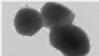
Ag Nanoparticles
