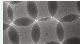
Silica Nanoparticles
